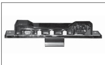
Invacare Full Electric Junction Box Accepts square, 4-pin plugs from motors (made after 7/98) or adapter cords.
